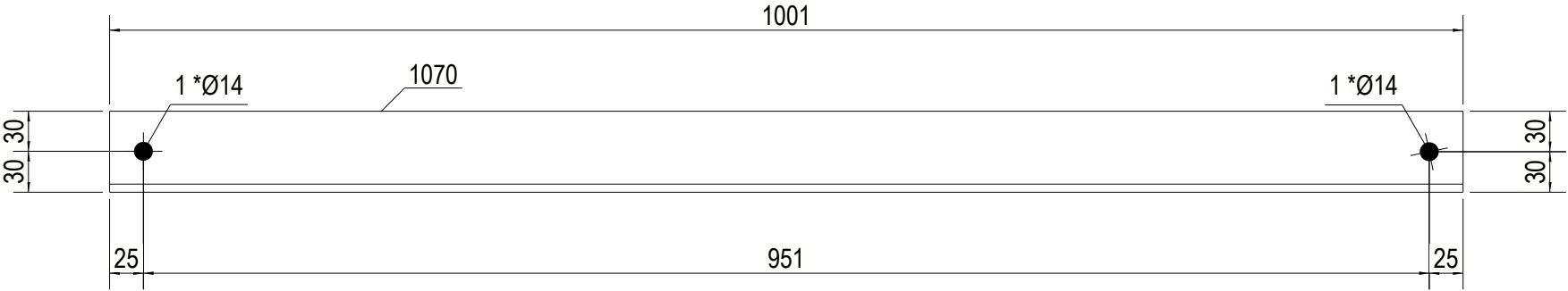
FRONT VIEW
